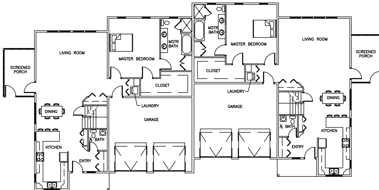
FIRST FLOOR 1490 S.F. Living Area
