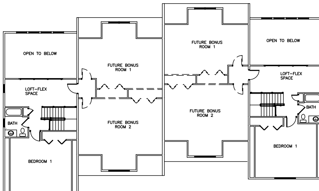
SECOND FLOOR 640 S.F. Finish Floor 875 S.F. 2 Future Bonus Rooms
